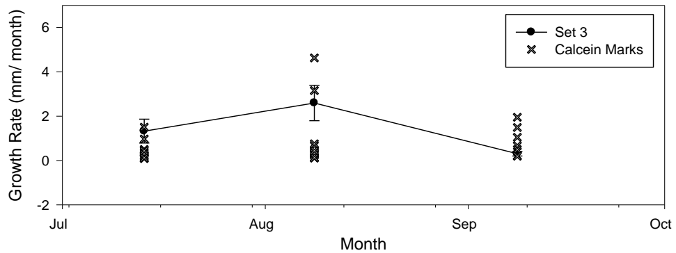
Figure 5. Growth rates measured during the summer of 2012 (set 3) by hand (black circles) and microscopically by calcein marks (gray x's).
