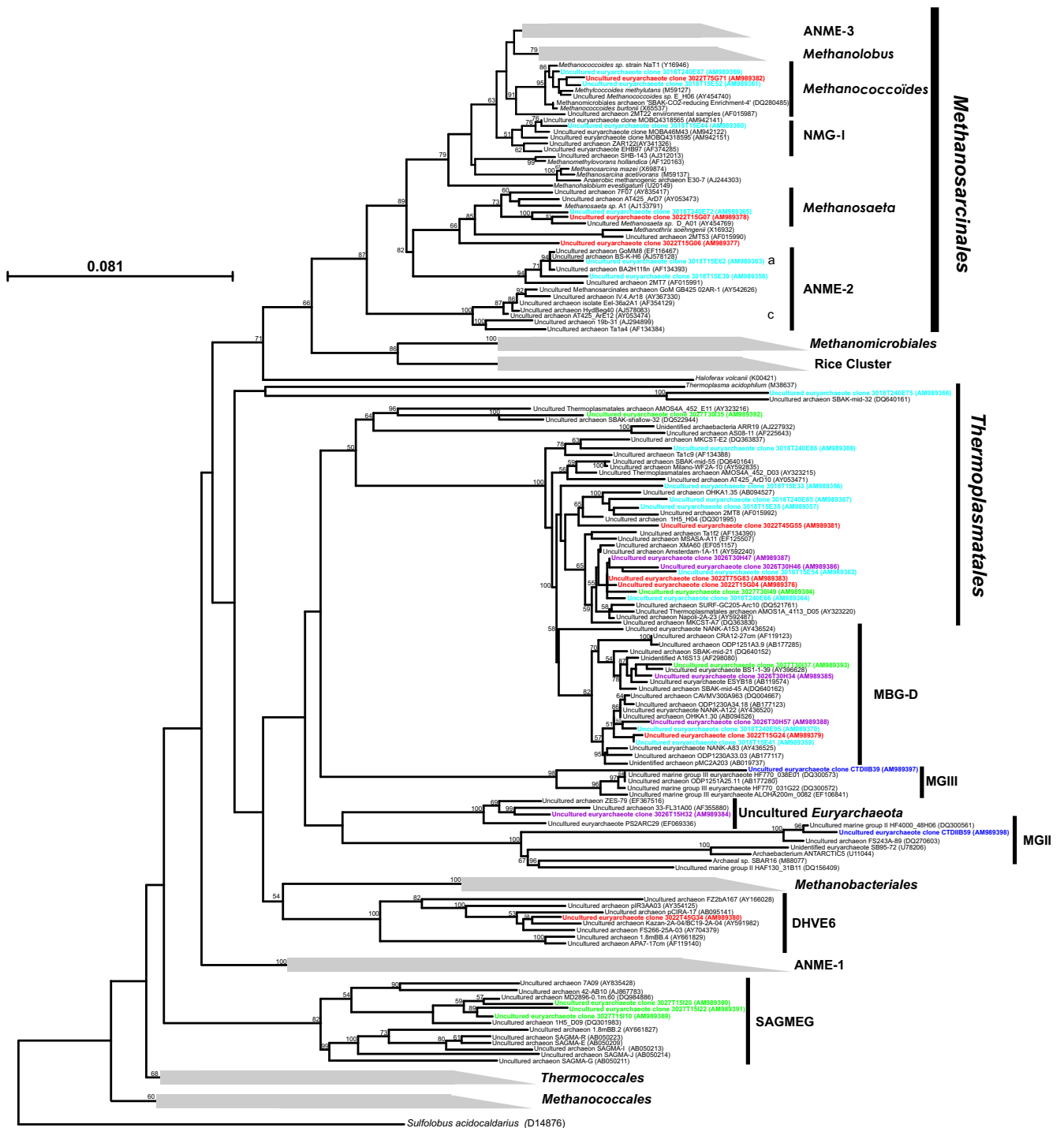
Fig. S3. Phylogenetic tree representing the Euryarchaeota 16S rRNA gene, except the Thermococcales lineage, sequences DNA- and RNA derived. RNA-derived sequences are underlined. Each phylotype is represented by one sequence with \geq 97\% similarity grouping. The tree was constructed using the neighbour-joining method with Jukes and Cantor correction. Bootstrap values < 50\% are not shown. ANME: anaerobic methane oxidizers, NMG-1: Novel Methanosarcinales group 1, SAGMEG: South African Gold Mine Euryarchaeotic Group, DHVE6: Deep-sea Hydrothermal Vent 6, MBG-D: Marine Benthic Group D, MG: marine groups.
