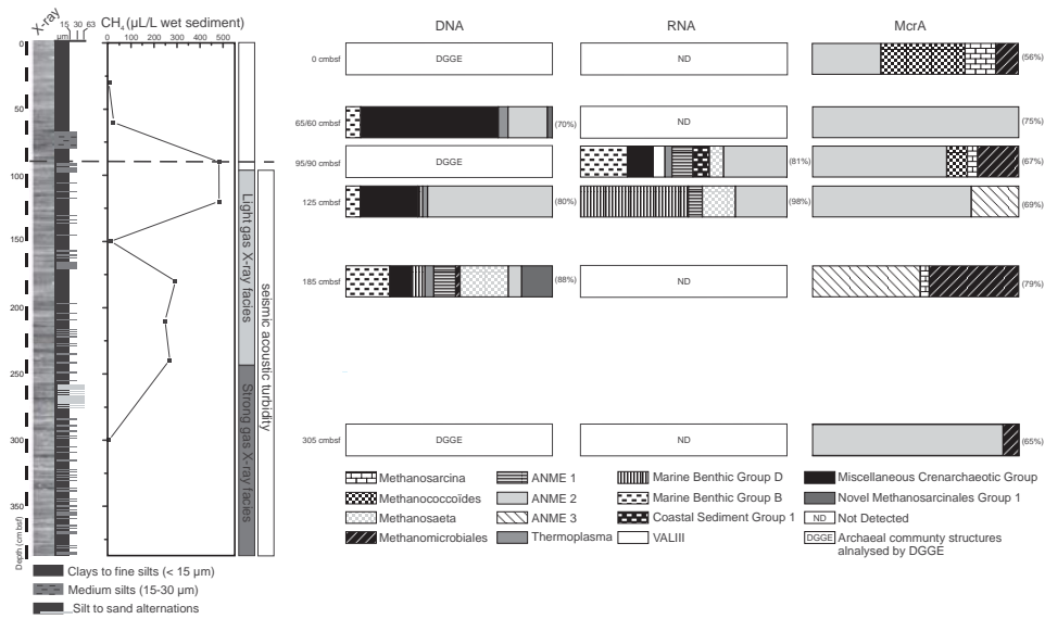
FIG. 2.4: Depth distribution of the archaeal phylogenetic community structures based on 16S rRNA, crRNA and mcrA gene compared to X-ray image, sedimentary facies and methane ( \text{CH}_4 ) concentration. The percentage of coverage of each clone library examined is indicated in brackets. The phylogenetic affiliation of each clone sequence was determined by similarity analysis. The relative abundance of each phylotypes in the clone library was calculated and represented in a column diagram. DNA designs the DNA-derived libraries; RNA, the RNA-libraries; McrA, the mcrA gene libraries.
