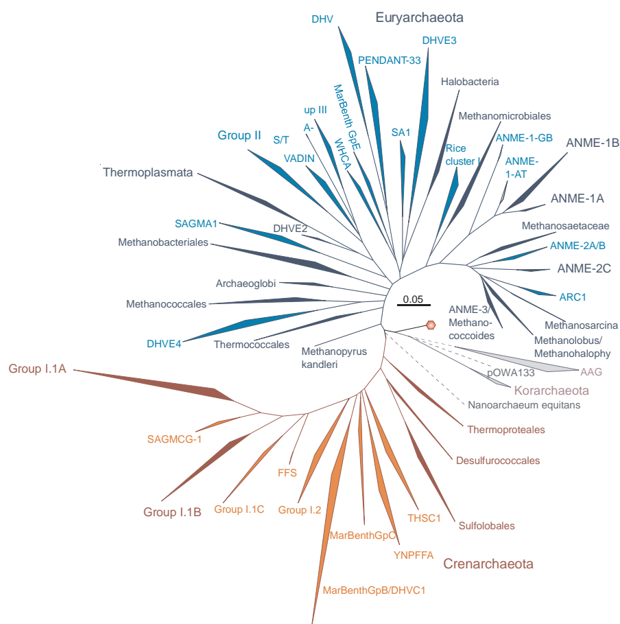
FIG. 1.24: The phylogenetic diversity of the domain of Archaea . Triangles in light colours represent branches with exclusively uncultivated species, dark triangles show branches with cultivated species. The size of the triangle is proportional to the number of sequences analysed. The red hexagon in the centre indicates rooting to species in the domain Bacteria . The phylogenetic tree is based on comparisons of 16S rRNA gene sequences from the Euryarchaeota , Crenarchaeota and Korarchaeota phyla together with Nanoarchaeum equitans (dotted lines indicate uncertain phylogenetic positions), clone pOWA133 and the ancient archaeal group (AAG), which are not classified within these phyla; modified from (Schleper et al. , 2005).
