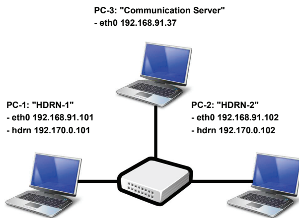
Figure 4.3: Experiment Setup
