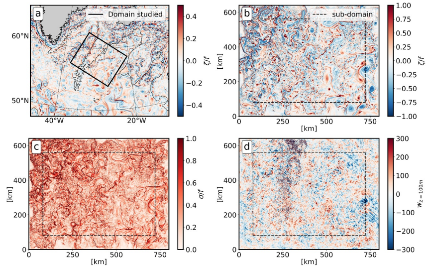
Figure 1. (a) Snapshot of the GIGATL3 simulation ( dx = 3 km) on the 8th of February. The background is the relative vorticity and the black contour is the bathymetry at 2,000 m. The black rectangle is the domain of the regional simulation. (b–d) represent the relative vorticity, the strain and vertical velocity at 100 m depth, respectively, computed from the regional simulation ( dx = 800 m). The relative vorticity and strain are normalized to the local Coriolis frequency. All the statistical results are computed in the dashed rectangle subdomain to discard boundary effects.
