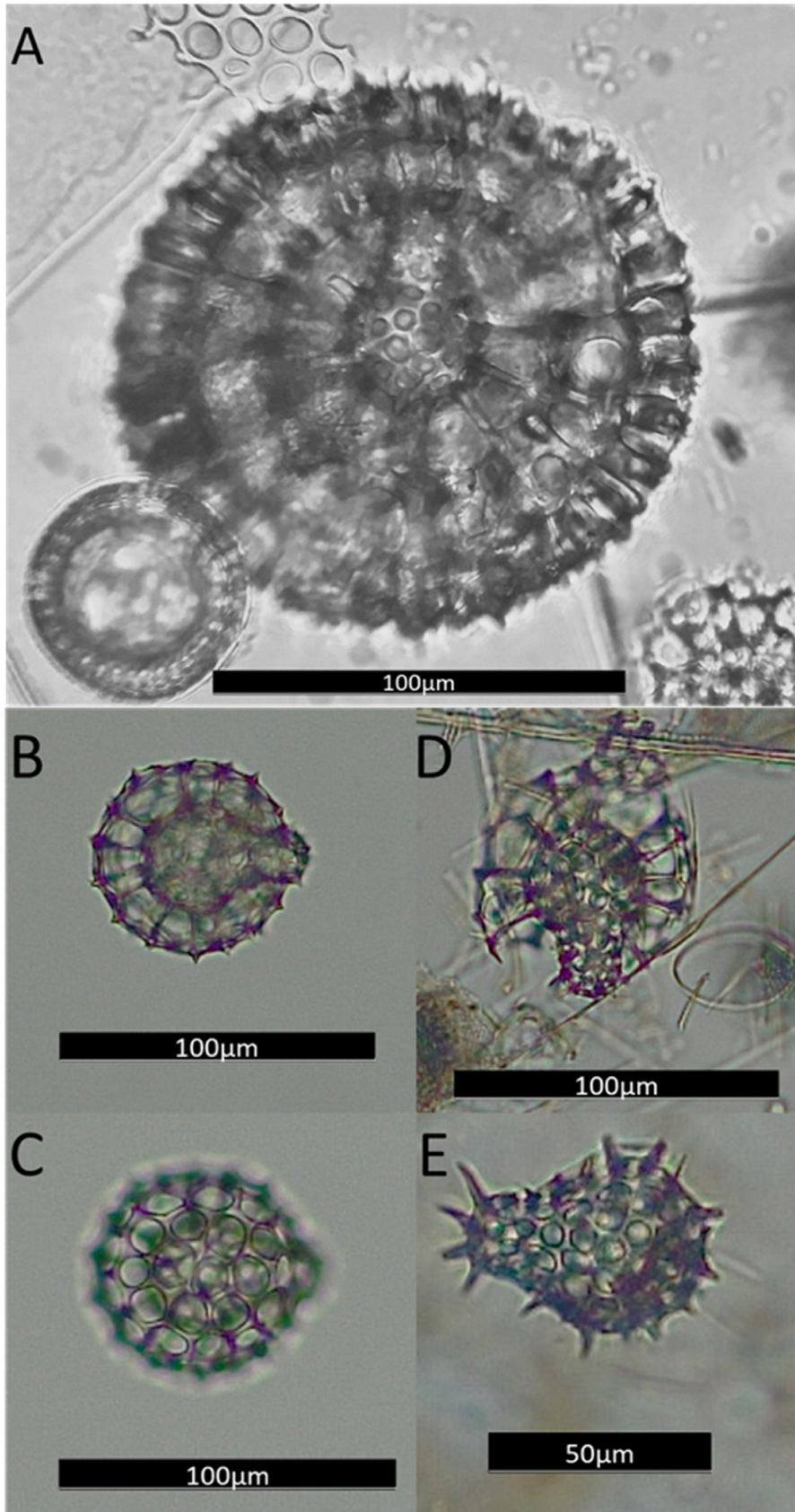
Plate 1. Pirumosphaera armandae A) holotype (core site MD19-3575CQ, 299-300 cm), most complete specimen; B & C) paratype 1 (core site TAN1302-97, 21-22 cm), same specimen at two focus levels, inner and 2nd shell present, 3rd and 4th shells missing; D) specimen with second shell broken (core site TAN1302-97, 171-172 cm); E) paratype 2, Specimen consisting of inner shell only with spines, all other shells missing (core site TAN1302-97, 191-192 cm).
