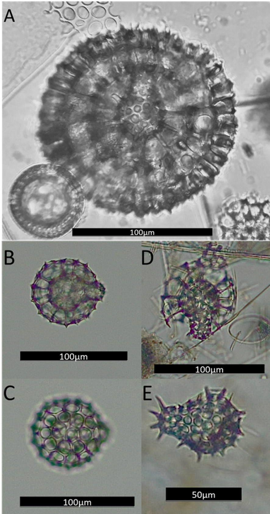
Plate 1. Pirumospaera armandae A) holotype (core site MD19-3575CQ, 299-300 cm), most complete specimen; B & C) paratype 1 (core site TAN1302-97, 21-22 cm), same specimen at two focus levels, inner and 2nd shell present, 3rd and 4th shells missing; D) specimen with second shell broken (core site TAN1302-97, 171-172 cm); E) paratype 2, Specimen consisting of inner shell only with spines, all other shells missing (core site TAN1302-97, 191-192 cm).
