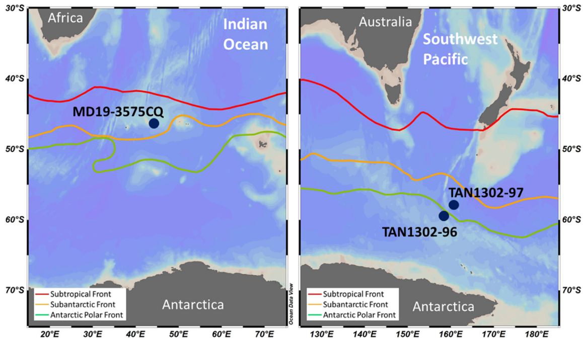
Fig. 1. Sediment core locations where specimens of the newly described species were recorded in the Southwest Pacific and Indian sectors of the SO. Fronts locations according to Orsi, 1995.
