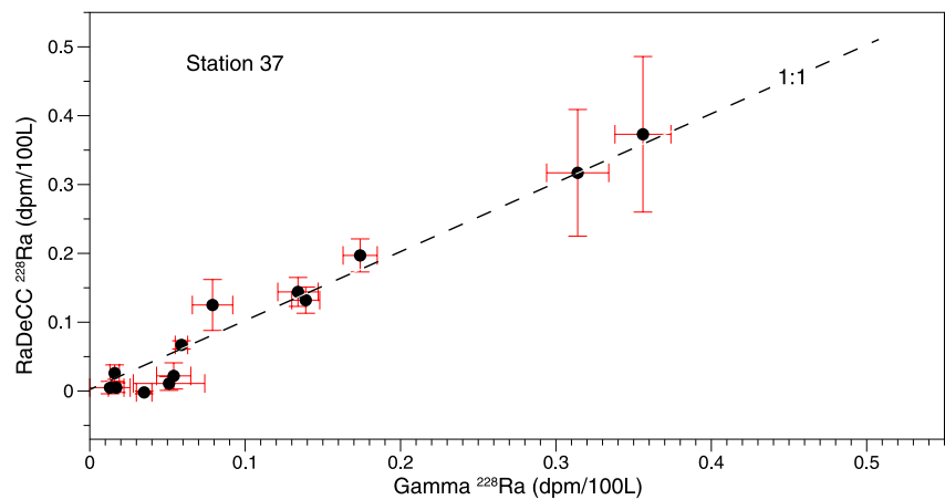
Figure 3. Comparison of ^{228}\text{Ra} at station 37 as determined by RaDeCC measurement followed by gamma ray spectrometry. Error bars are 1 sigma. Corrected to time of collection.
