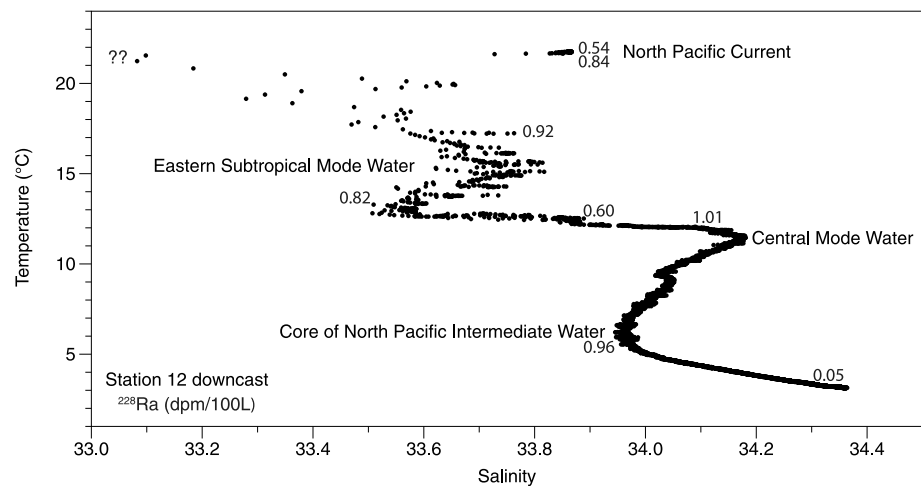
Figure 7. Upper (0–1,000 m) water column profile of temperature and salinity at Station 12 (37°N, 152°W). The water masses are identified and ^{228}\text{Ra} activities (dpm/100 L) are indicated.
