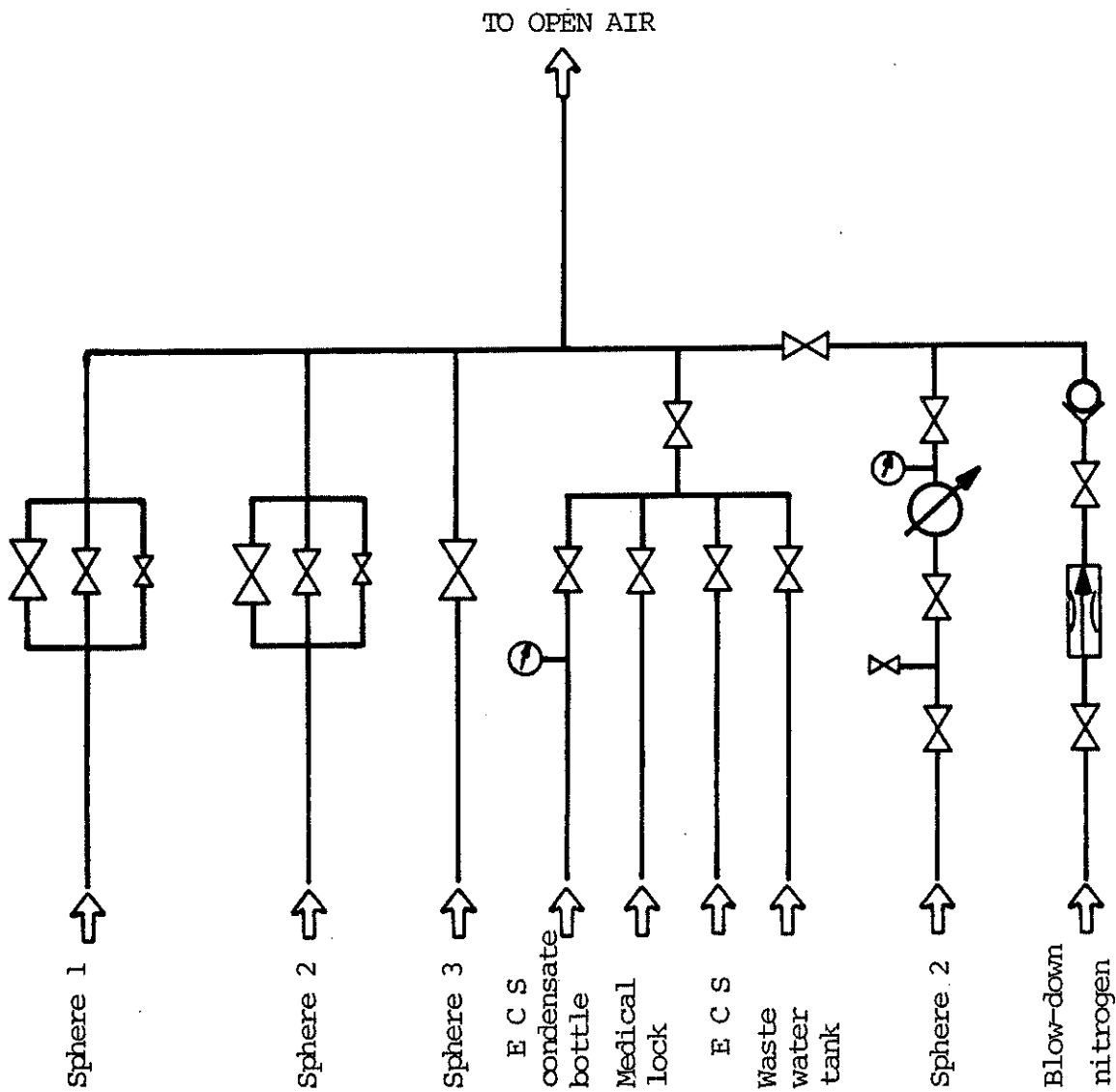
Figure 15 : EMS 600 decompression circuit diagram
