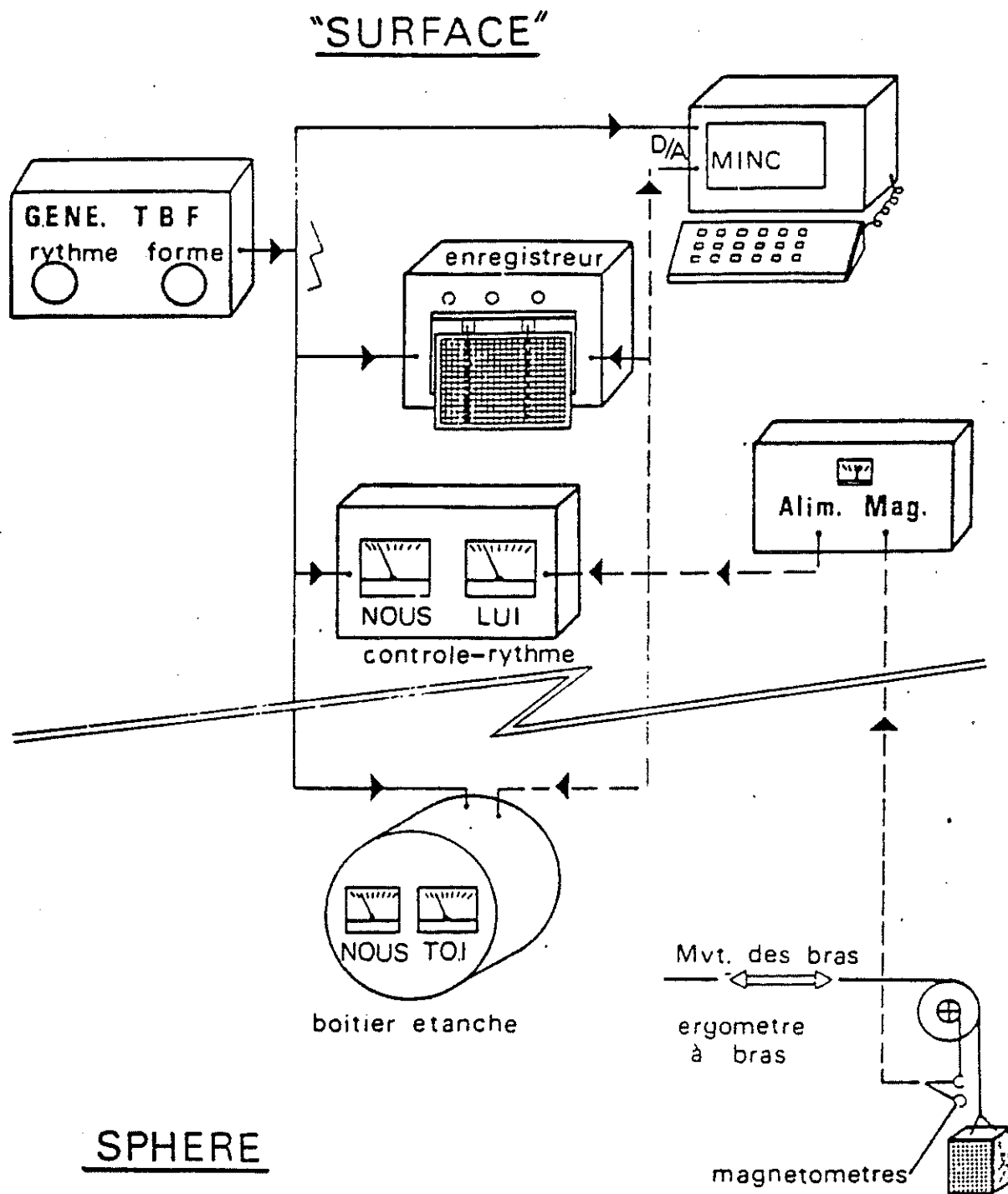
Figure 1. TRANSMISSION OF THE EXERCISE RYTHM TO THE DIVER AND THE MONITORING OF ITS EXECUTION
