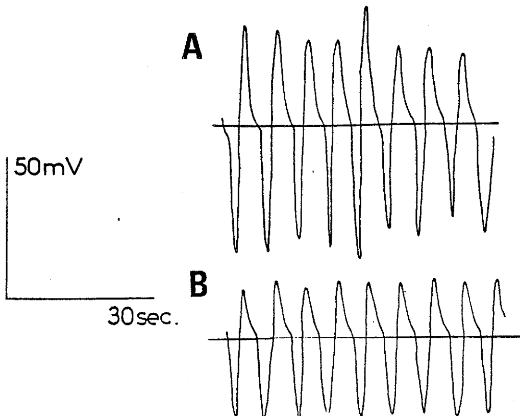
Figure 3 SIGNAL DERIVED FROM THE MASS FLOWMETER AT 46 BAR
