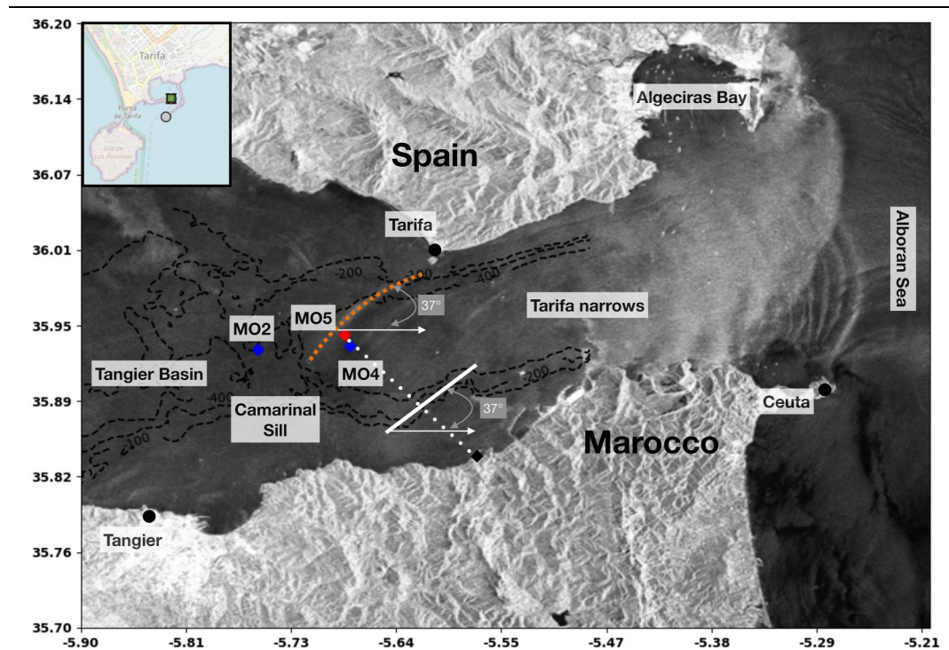
Figure 1. Map of the studied area over Sentinel-1 Synthetic Aperture Radar (SAR) image. Black dashed lines show few isobaths in the western part of the domain. Blue diamonds correspond to MO2, MO4 Acoustic Doppler Current Profilers moorings, red diamond corresponds to MO5 CT mooring. Orange dashed line shape the R-wave of the SAR image (see text). White line is the spatially averaged tangent of the isobaths along the Moroccan shelf, which is oriented 37^\circ with respect to the east (gray text). White dotted line corresponds to the section used in the numerical approach (see Section 5). Inset: Zoom on Tarifa harbor, the green squared depicting the location of the tide gauge.
