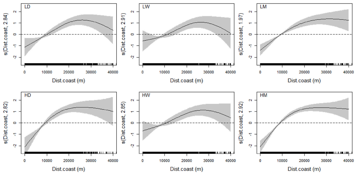
Fig. 6. Smoothers for distance to the coast , variable selected in all the final GAMs for fin whales. LD = Low resolution daily model. LW = Low resolution weekly model. LM = Low resolution monthly model. HD = High resolution daily model. HW = High resolution weekly model. HM = High resolution monthly model. Black marks on the x-axis indicate the distribution of the observations.
