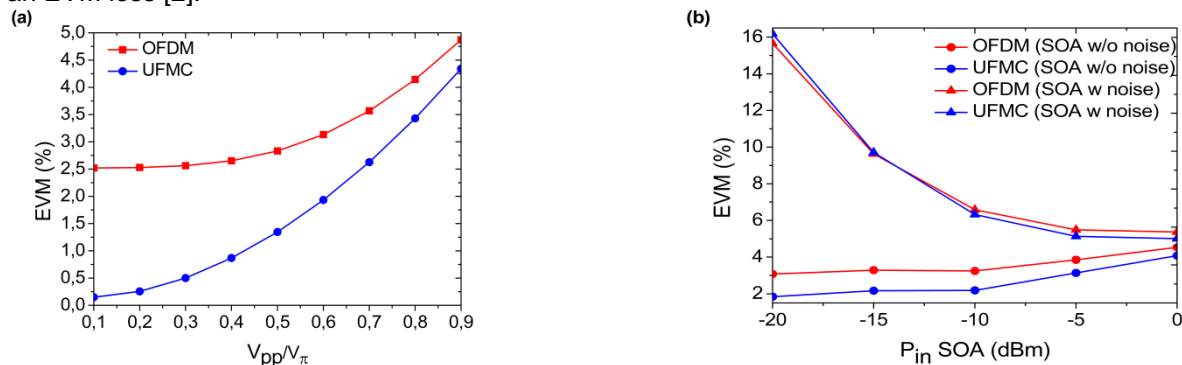
Figure 2. Average EVM performance for 3 OFDM/UFMC bands (a) vs V_{pp}/V_{\pi} (w/o SOA); (b) vs P_{in\ SOA} (w SOA).
