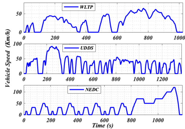
Figure 3. Speed profiles.
