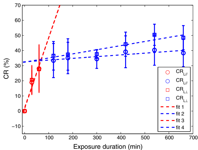
Fig. 5 Variation of speckle contrast ratio (CR) as a function of duration of tooth exposure to acid (in minutes). Error bars correspond to the standard deviation. CR_{L//} and CR_{L\perp} are related to the linear co- and cross-polarized analysis configuration, respectively. Symbols correspond to experimental data. Lines are guides for the eyes.
