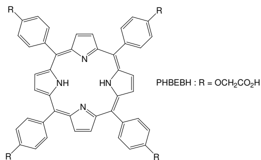
Fig. 32. Structure of 5,10,15,20-tetrakis[4-carboxymethyleneoxyphenyl]porphyrin (PHBEPH). PHBEPH : R = \text{OCH}_2\text{CO}_2\text{H}
