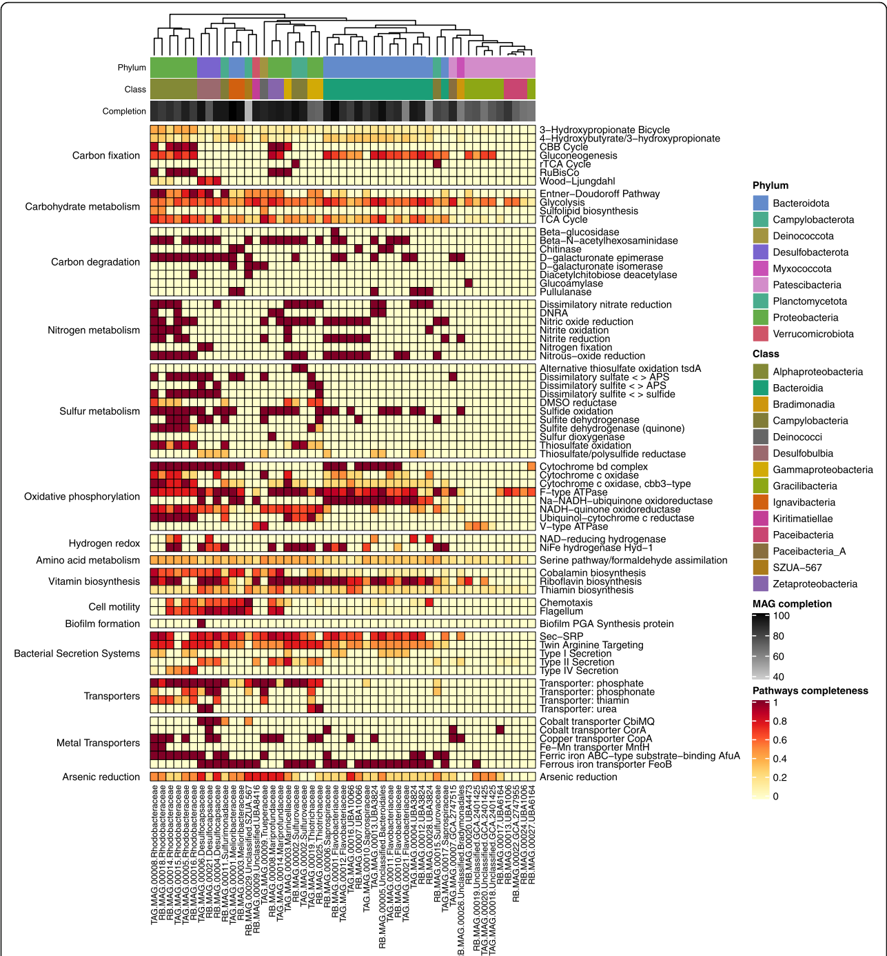
Fig. 5 KEGG Decoder heat map based on KEGG annotation. The heat map represents metabolic pathway completeness of the MAGs based on the presence or absence of genes as determined by KEGG Decoder. The data represent the discussed pathways, all of which are shown in Additional File 15. The dendrogram at the top represents the similarity between the MAGs based on their metabolic pathways, using Euclidean distance and complete linkage clustering. Taxonomic affiliations at the class and phylum levels are indicated and represented by the different colors. NAD-reducing hydrogenase, hoxHFUY ; NiFe hydrogenase Hyd-1, hyaABC
