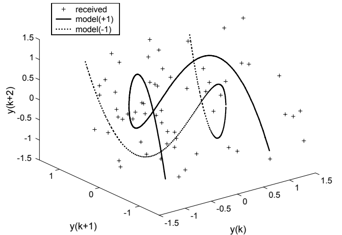
Figure 3: Representation of vectors \mathbf{y}_k and symbolic models \mathbf{z}_{+1}(x) and \mathbf{z}_{-1}(x) in a 3-dimensional space ( N = 3 ). The map is g(x) = 1 - 2x^2 and the signal to noise ratio is SNR = 3dB .
