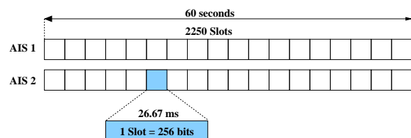
Figure 1: AIS frame organization in TDMA mode
