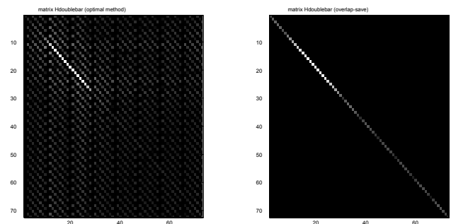
Figure 6: Bidimensional frequency response (matrix \overline{\overline{H}} ). Left: optimal method. Right: overlap-save.
