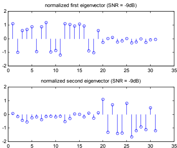
Figure 2: Normalized eigenvectors
