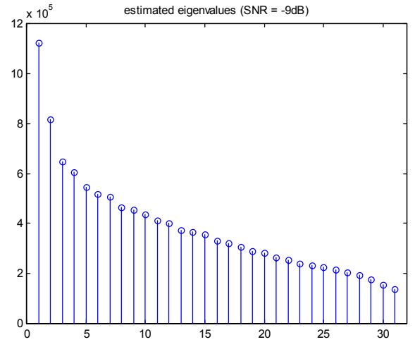
Figure 1: Estimated eigenvalues
