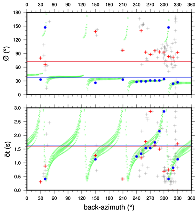
Figure 4. Results at station GOGA for synthetic SKS (blue circles) and XKS observed data (gray crosses) splitting parameters in functions of back azimuth. Red crosses represent the average value for observed data for a 10^\circ back azimuth interval. Upper panel represents the polarization direction of the fast S wave, and lower panel corresponds to the time delay between the fast and the slow S waves. As an indication, splitting parameters of the average layer model for synthetic (blue line) and observed data (red line) are represented. The light green circles represent the best model after inversion of the synthetic SKS.
