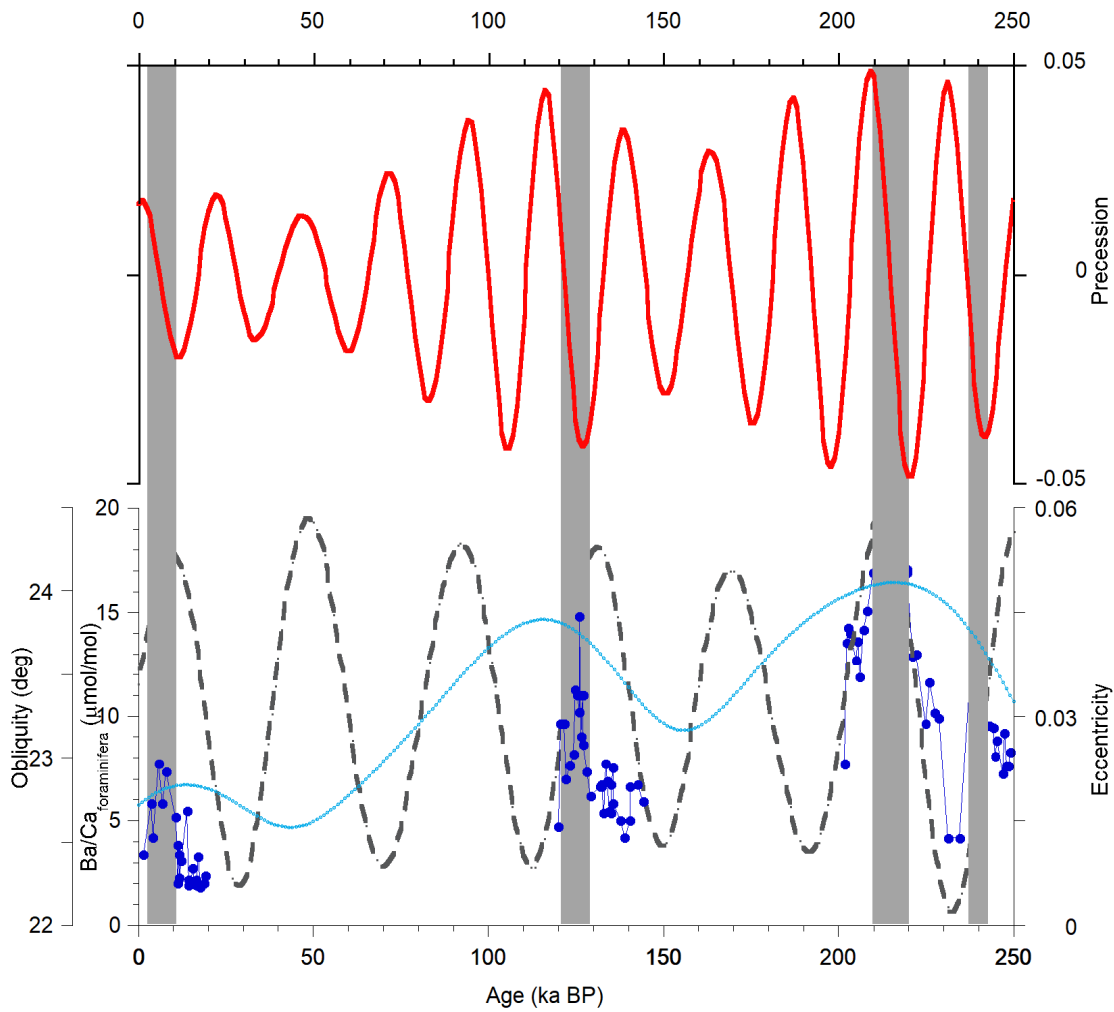
940 Figure 5. Comparison of Ba/Ca (runoff/rainfall) record (deep blue) with orbital forcing; Obliquity (grey dashed curve), eccentricity (light blue) and precession (red). Grey bands indicate warm periods MIS 7, 5 and MIS 1. Changes in the amplitude of Ba/Ca follows the eccentricity cycle, with higher Ba/Ca during MIS-7, relatively lower Ba/Ca in MIS-5, and the lowest Ba/Ca in MIS-1, corresponding to the respective insolation maxima of the 100 ka-eccentricity cycle during each interglacial. This trend in the change in magnitude of river discharge due to winter rainfall confirms the idea of eccentricity 945 modulation of the precession-driven rainfall/runoff in the Mediterranean during the late Pleistocene.
