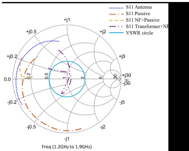
Fig. 16 Step-by-step wideband matching for the 3 rd topology
