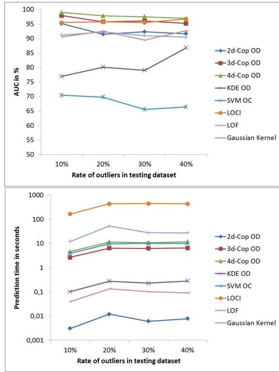
Figure 22: Average calculated AUC and prediction time for the Intel Berkeley dataset with different rates of outliers in testing dataset, five runs of Monte Carlo cross validation.
