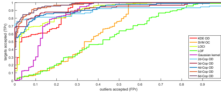
Figure 19: ROC plot for the Saint Bernard dataset with 30% of outliers in both the training and the testing datasets.
