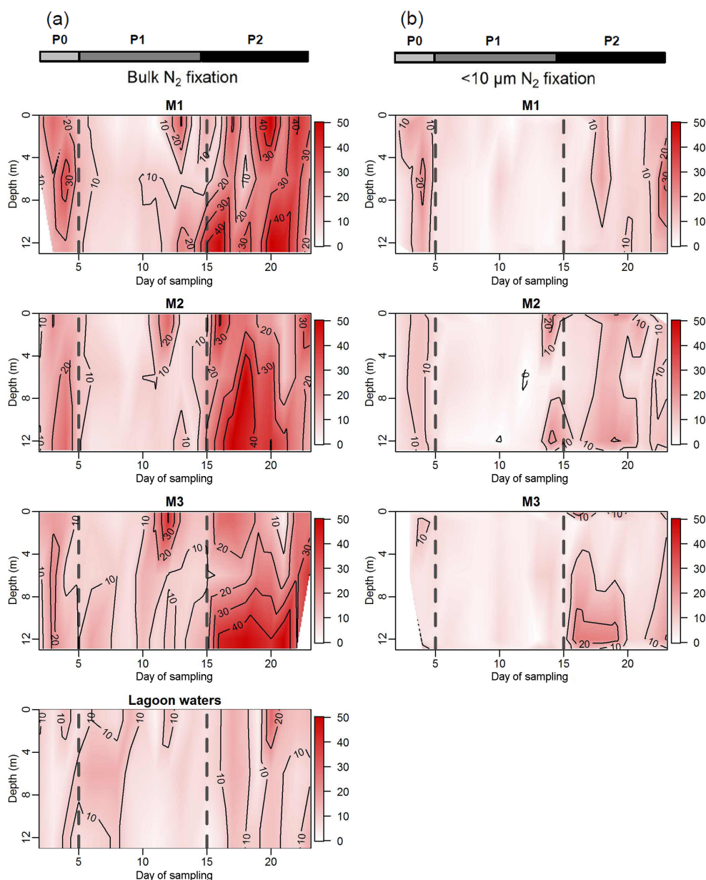
Figure 2. (a) Horizontal and vertical distributions of bulk N 2 fixation rates (nmol N L -1 d -1 ) in M1, M2, M3 and lagoon waters, and (b) <10 μm N 2 fixation rates (nmol N L -1 d -1 ) in M1, M2, and M3. Note that N 2 fixation rates in the <10 μm fraction were not measured in lagoon waters.
