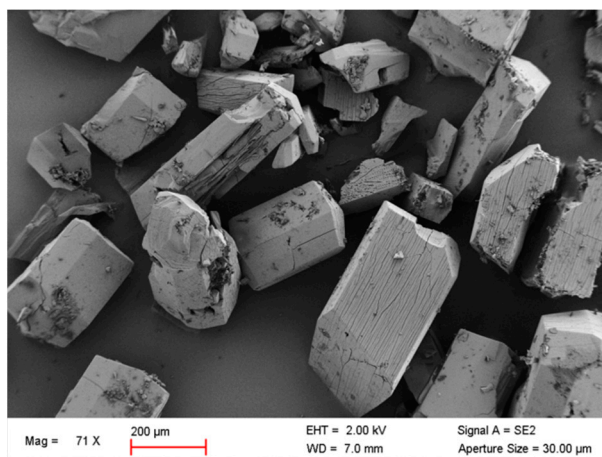
Figure 6. SEM image of showing the morphology of \text{Mn}(\text{H}_2\text{O})_2[\text{O}_2(\text{OH})\text{PC}_{15}\text{H}_{13}]_2 \cdot 2\text{H}_2\text{O} .
