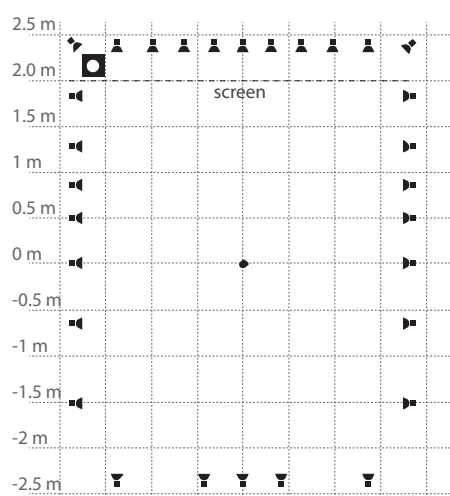
Figure 1: Loudspeaker configuration
