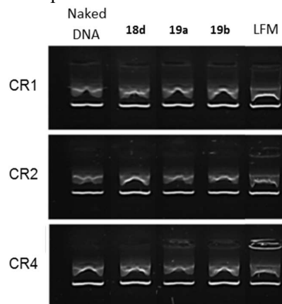
Figure 4. DNA complexation ability of compound 18d (formulated with DOPE) as determined via the agarose gel retardation assay for different charge ratios. Previously synthesized quaternary ammonium sophorolipids 19a and 19b , naked DNA and LFM (Lipofectamine 3000) were used as controls.
