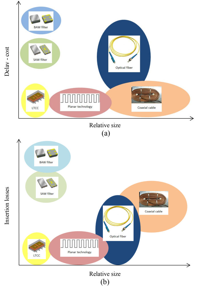
Fig. 2. State-of-the-art technologies: (a) Delay and cost vs Size, (b) Insertion losses vs Size.
