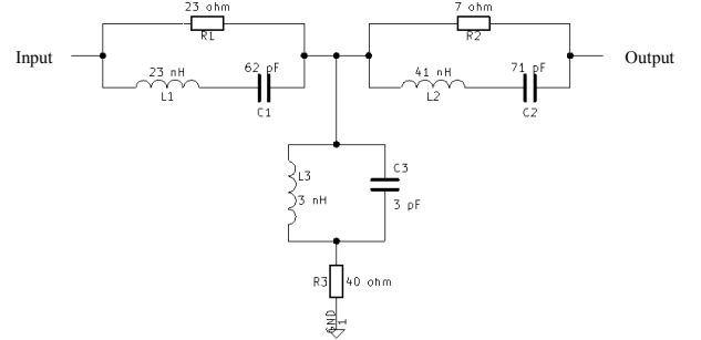
Fig. 4. Topology of a non-reflective filter.
