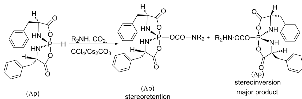
Scheme 20: AT reaction with hydrospirophosphorane with insertion of CO 2 in the product (adapted from [69]).
