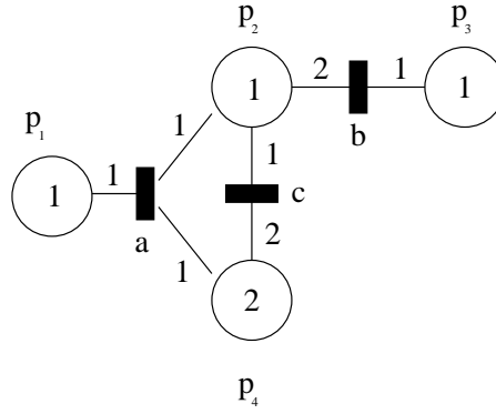
Figure 1: A strict- \mathbb{Z}/3\mathbb{Z} -net
