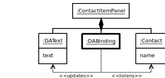
FIGURE 10. Using of a DABinding
