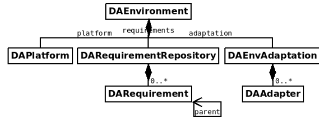
FIGURE 11. The environment composition
