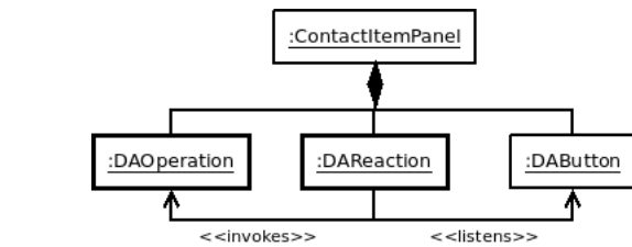
FIGURE 9. Using of a DAResponse
