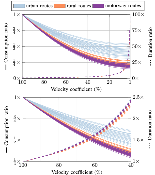
Fig. 2. Evolution of the routes ratios on (a) the complete domain of velocity coefficients and on (b) a domain restricted to [40\%; 100\%] .
