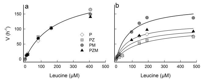
Fig. 9. Aminopeptidase activity in the background water of the tanks on days 0 (a) and 8 (b) as determined from the hydrolysis of leucine. The values of V_{\text{max}} and K_s for the curve shown in (a) are 227 \pm 10 \text{ h}^{-1} and 192 \pm 18 \mu\text{M} ( r^2 = 0.99 ). In (b), the highest curve (the one for PM) has a V_{\text{max}} of 177 \pm 19 \text{ h}^{-1} and a K_s of 87 \pm 28 \mu\text{M} ( r^2 = 0.97 ), while the lowest curve (the one for PZ) has a V_{\text{max}} of 103 \pm 14 \text{ h}^{-1} and a K_s of 157 \pm 50 \mu\text{M} ( r^2 = 0.98 ).
