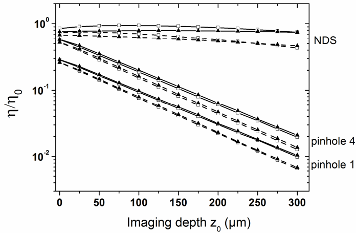
Fig. 2. Monte Carlo simulations of the z-profile of collection efficiencies \eta_{\text{conf}} (pinhole 1 and 4) and \eta_{\text{NDS}} , without absorption (full lines) and with absorption \mu_a = 10\text{cm}^{-1} (dashed lines), for g = 0.85 (empty square) and g = 0.95 (full triangle). The vertical scale is logarithmic and \mu_s = 100\text{cm}^{-1} .
