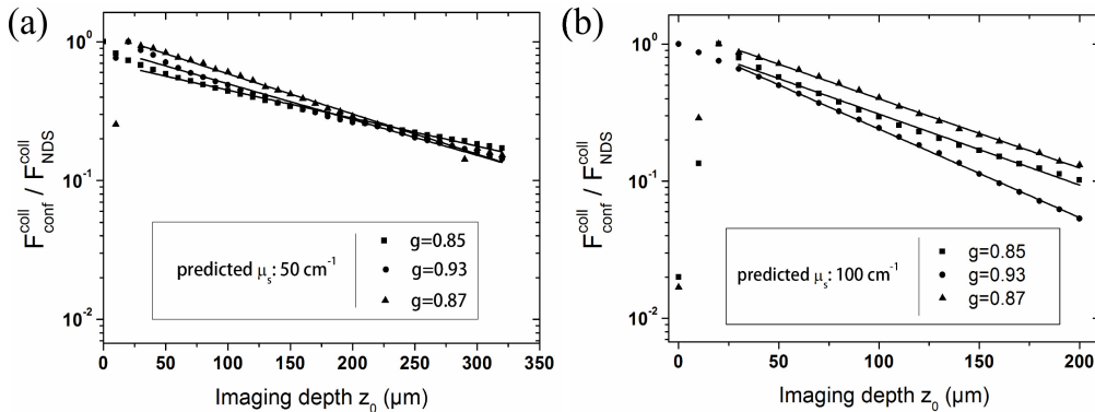
Fig. 6. Semi-log representation of the confocal-to-nondescanned ratios of the two-photon excitation fluorescence intensity versus imaging depth measured from six scattering gels with scattering coefficients of \sim 50\text{cm}^{-1} and \sim 100\text{cm}^{-1} , and three distinct anisotropy factors (see Table 4). The confocal pinhole has a diameter of 200\mu\text{m} (pinhole 4). Straight lines stand for linear fits of experimental data (dots), allowing to determine the true scattering coefficients through Eq. (4).
