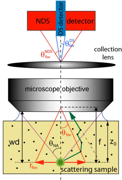
Fig. 1. Geometry of the collection paths used in the Monte Carlo simulations and useful parameters. f : focal length of the objective; w_d : working distance; \theta_{\text{NA}} : numerical aperture angle; r_{\text{fov}} : linear field of view; \theta_{\text{fov}}^{\text{DS}} and \theta_{\text{fov}}^{\text{NDS}} : angular field of view of the confocal (or descanned DS) and non-descanned NDS ports, respectively.
