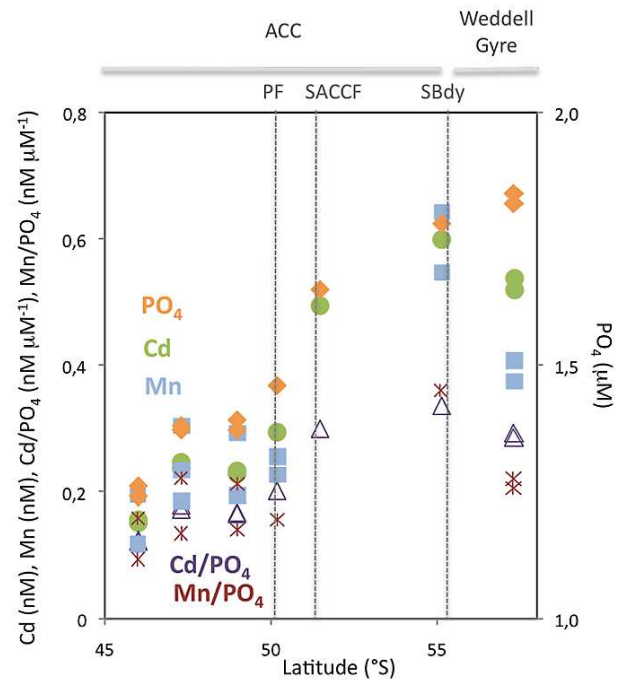
Fig. 8. Variations of Cd (green circles, in nM), Mn (blue squares, in nM) and \text{PO}_4 (orange diamonds, in \mu\text{M} ) concentrations, and of Cd/ \text{PO}_4 (purple triangles) and Mn/ \text{PO}_4 (dark red crosses) ratios (in \text{nM g } \mu\text{M}^{-1} ) as a function of latitude in the surface waters ( > 60 \text{ m} ) of the Antarctic Circumpolar Current and the northern Weddell Gyre along the Greenwich Meridian.
