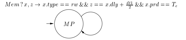
Figure 12. The test model of the measurement point MP (functional model with an added testing strategy)
