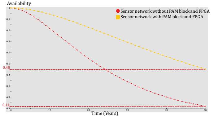
Fig. 9. Comparison of network availability with and without our approach
