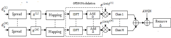
Figure 1. Transmitter structure of an OFDM-IDMA scheme with M simultaneous users
