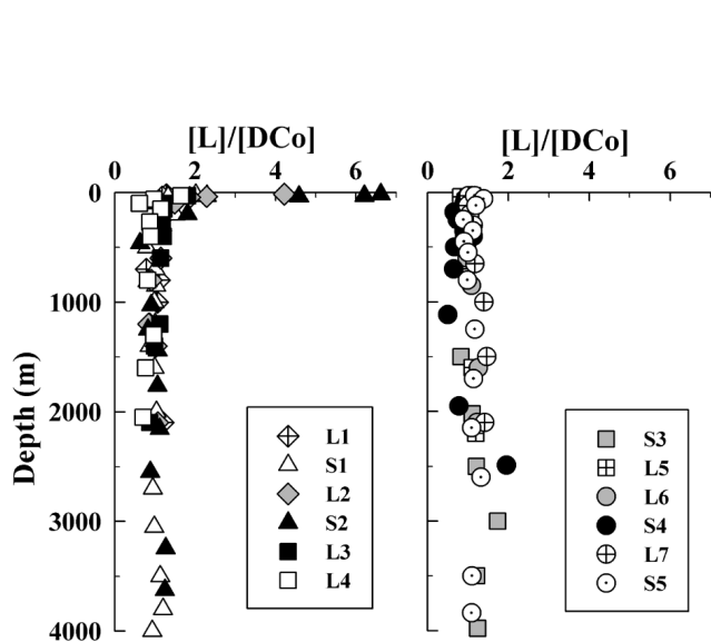
Fig. 4. Vertical distribution of L/DCo picomolar ratios in the subtropical and subantarctic domains (left panel), and in the polar frontal zone, the southern ACC and the northern Weddell Gyre (right panel).
