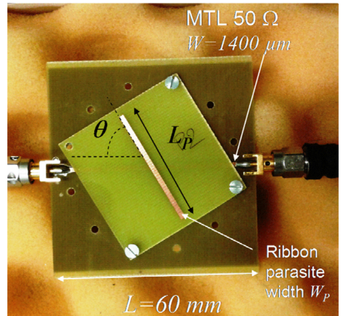
Fig. 1: Top view of the structure under test– Microstrip line (MTL) in the presence of a disturbing floating metal strip.
