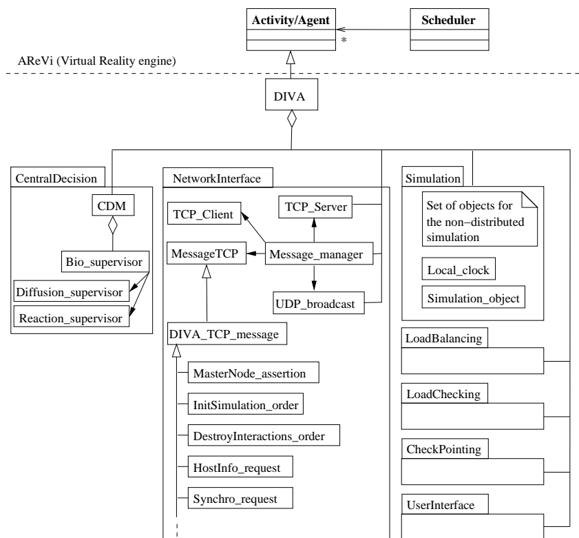
Figure 3. Simplified UML class diagram of the DIVA software.
