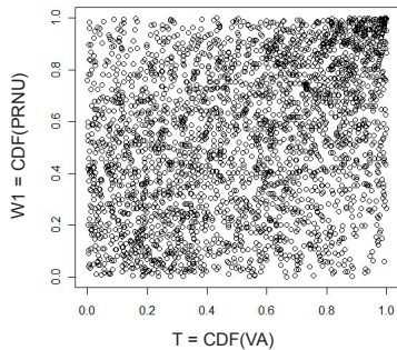
Fig. 7. 3000 samples of the empirical copula of the PRNU and VA.
