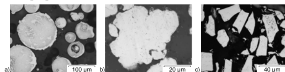
Fig. 1: Micrographs of used soft magnetic powders: a) gas atomized FeSi6.8, b) water atomized Fe, c) milled Fe_{73.5}Si_{15.5}B_7Cu_1Nb_3 ribbons
