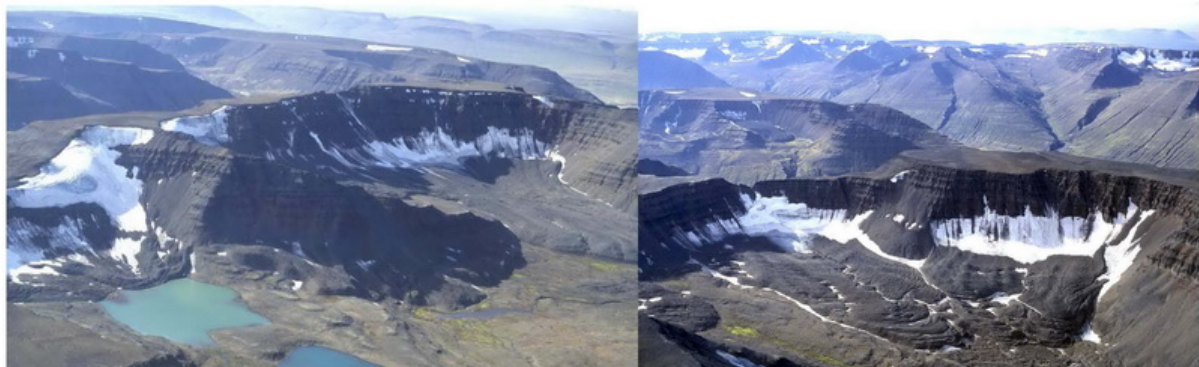
Figure 1. Composite talus derived and glacial derived rock glaciers near Holar in Tröllaskagi.
