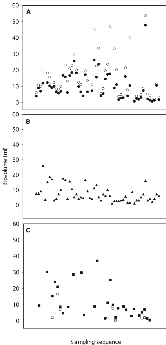
Fig. 3. Biovolume (ml) estimated from LOPC (A), with the volumetric method (B), the Zooscan and the microscope (both in panel C). LOPC-BB (○); LOPC-BB 500 (●); TPV (▲); Zooscan (■); Microscope (□). Data are aligned along the x axis following the sampling sequence. See text for further explanation.
