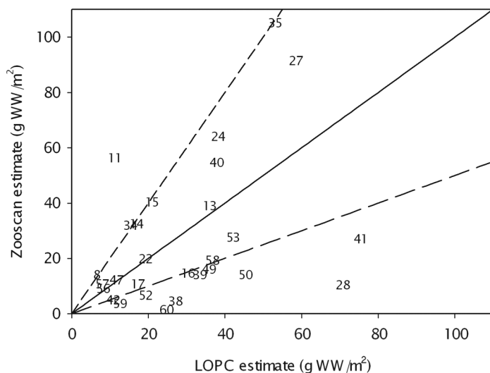
Fig. 5. Comparison of areal biomass (g wet weight/m 2 ) estimated by the Zooscan and the LOPC (>500 μm ESD). Numbers on graph indicate the station number. The 1:1 line and the range within the LOPC and the Zooscan agree within a factor of two (dashed lines).
