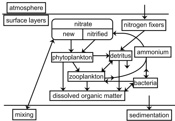
Figure 1. Schematic of the model used in the study. The split nitrate pool and nitrification are described in the text. Otherwise, model details, including equations, are given by Anderson and Pondaven [2003]. Note that the nitrogen taken up by nitrogen fixers only appears in the model on their demise and subsequent transition to detritus.
