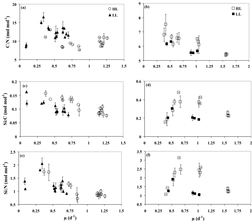
Fig. 4. Molar ratios of C:N (a, b), Si:C (c, d) and Si:N (e, f) versus specific growth rate ( \mu , d -1 ) of Thalassiosira oceanica (left panels) and Ditylum brightwellii (right panels) under high light (HL, open symbols) and low light (LL, closed symbols).
