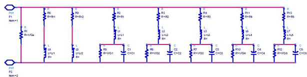
Fig.3b – Equivalent circuit for y_1
