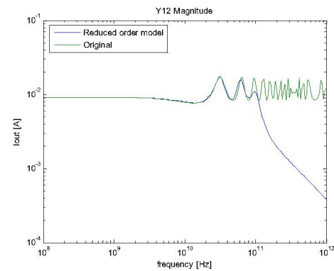
Fig.2c – Y_{12} , magnitude
