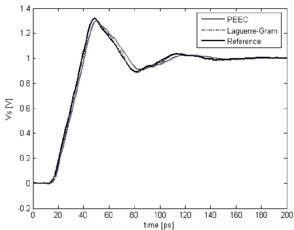
Fig.4 – Transient responses
