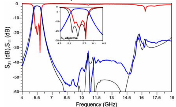
Figure 5: Experimental (thick lines) and EM ( S_{21} in thin line) simulated S-parameters. In-band measured parameters (thick lines) compared to the objective S_{21} parameter (thin line).
