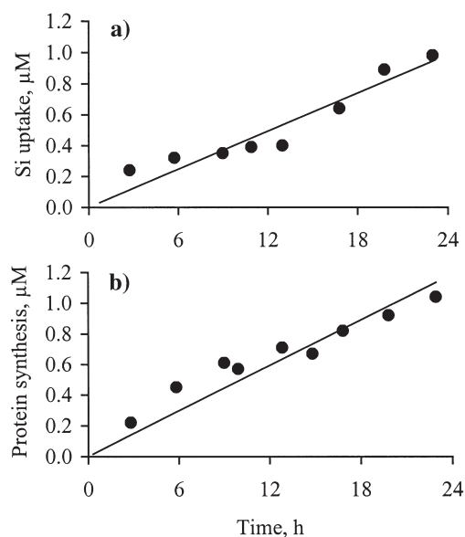
Fig. 5. Time course experiments of ^{32}\text{Si} uptake (a) and ^{14}\text{C} incorporation into proteins (b) by a diatom community (Assemblage 1) sampled in February 1995. C biomass was 8 \text{ mg C m}^{-3} and silicic acid concentration was 19.6 \text{ µM}
