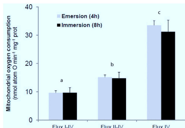
Fig. 3. Oxygen uptake related to electron flux through complexes I-IV, II-IV and IV of isolated mitochondria from gills of oysters sampled after 4 h of emersion or after 8 h of immersion. Assay temperature was 10 °C. Values are mean \pm SE ( n = 9 pools of 5 oysters for emersion and n = 6 pools of 5 oysters for immersion). Different superscript letters indicate values that differ between flux. Maximal flux through complexes of the ETC did not differ statistically between groups ( p < 0.05 ).
